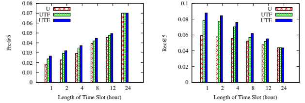
Figure 9: Performance of varying length of time slot
