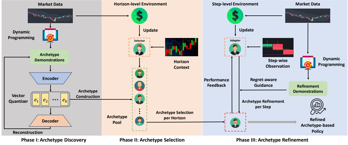
Figure 1: The overview of ArchetypeTrader: Phase I discovers meaningful and reusable strategic archetypes from demonstration trajectories using vector-quantized encoder-decoder. Phase II trains an archetype selector to choose archetypes based on horizon context. Phase III trains a regret-aware archetype adapter to refine the base archetype policy, guided by hindsight-optimal demonstrations.
