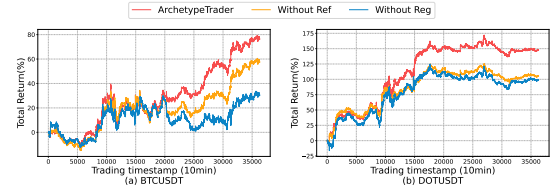
Figure 3: Performance of ArchetypeTrader and two variations of different refinement methods
