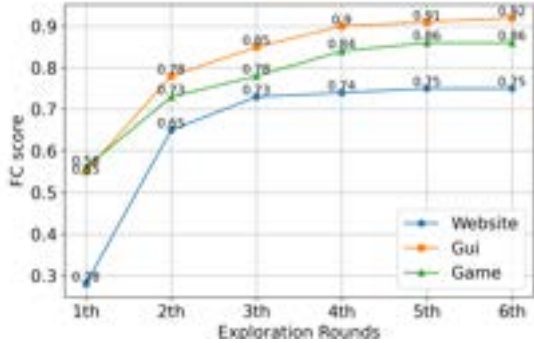
Figure 5: The FC score of each exploration round.
