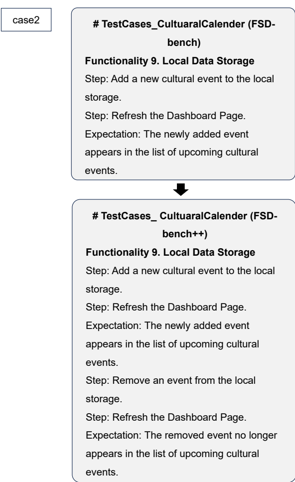
Figure 7: Example2 of additional test cases introduced in FSD-Bench++.
