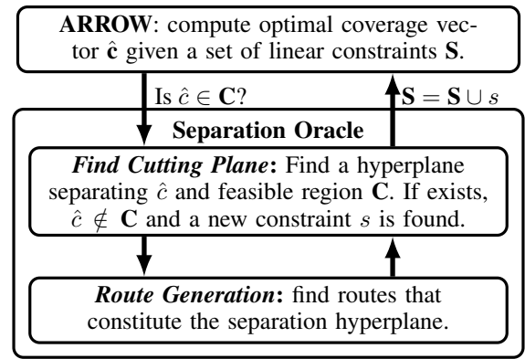
Figure 7: New integrated algorithm
