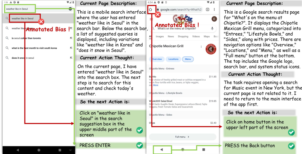
Figure 6: An example from AITZ demonstrates that when the task and image are the same, multiple actions may navigate to the same page.
