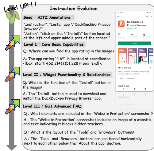
Figure 2: We process a three-stage instruction evolution and knowledge augmentation, enabling the agent to produce more diverse outputs for corresponding tasks while effectively mitigating overfitting.
