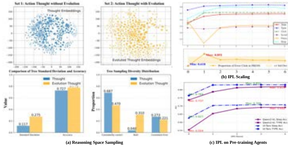
Figure 3: (a) Reasoning diversity before and after instruction evolution (left top) and the distribution of standard deviation and accuracy (left bottom). (b) Step.Acc changes for action types in AITZ across IPL iterations (right top). (c) The performance of UI-Tars-7B and Qwen2-VL-7B on AITZ as the seed model with 4-round IPL training (right bottom).
