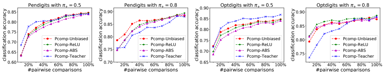
Figure 1. The classification accuracy of our proposed Pcomp classification methods when the number of pairwise comparisons increases.
