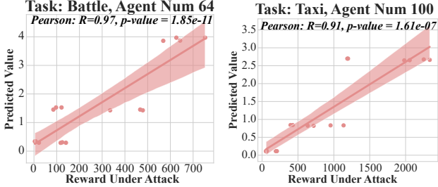
Figure 2. Pearson correlation between the lower-level attack value estimated by our Bellman operator \mathcal{B}_{\epsilon^i, \xi}^R (y axis) and lower-level reward by running an attack using RL (x axis). Our proposed Bellman operator is an accurate predictor of attack result.
