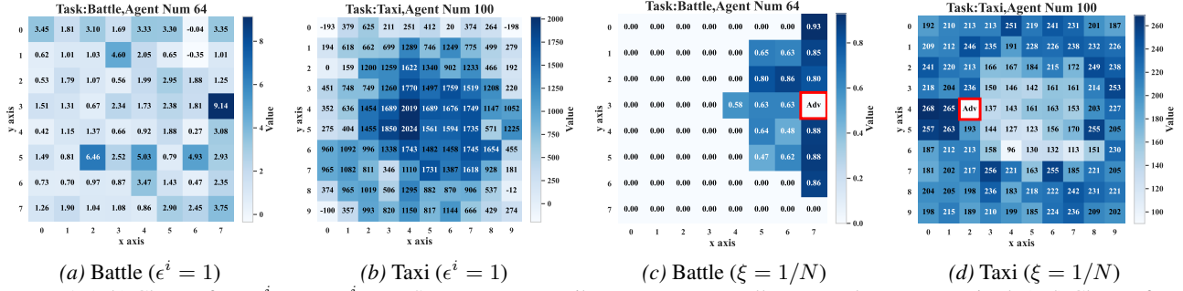
Figure 1. (a,b) Change from \epsilon^i = 0 to \epsilon^i = 1 . Some agents contribute more to overall system when compromised. (c,d) Change from \xi = 0 to \xi = 1/N . Agents receive more impact when facing attackers. Darker cell indicates higher vulnerability.
