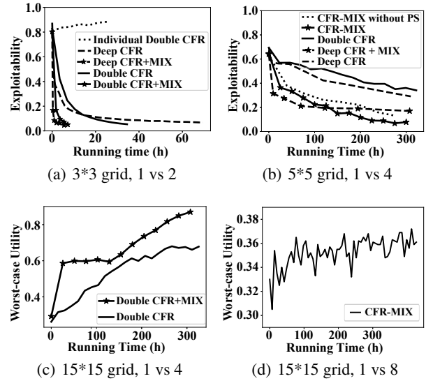
Figure 4: NEST Games
