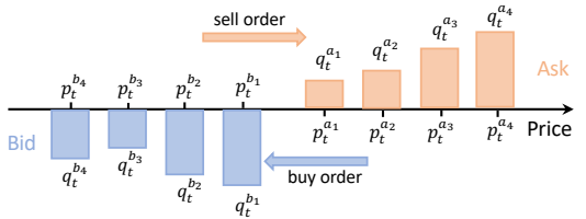
Fig. 3. A Snapshot of Limit Order Book.
