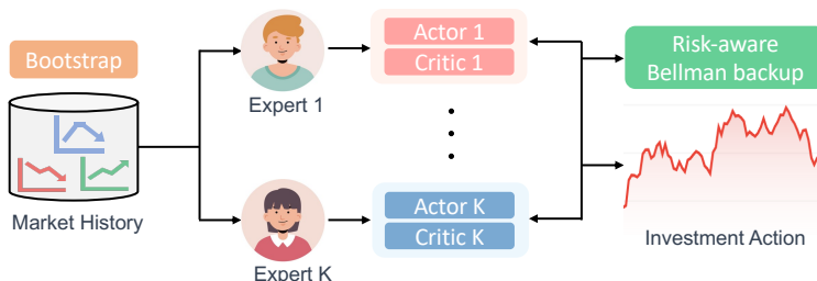
Figure 3: An illustration of AlphaMix+, a universal deep RL framework with diversified risk-aware mixture-of-experts.
