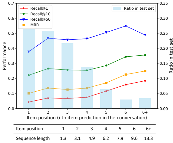
Figure 2: The performance of TSCR with the ordinal number of item predictions.
