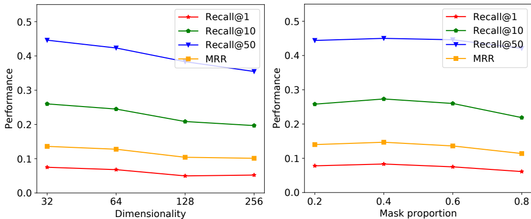
Figure 3: Effect of hidden dimensionality (left) and mask proportion (right).
