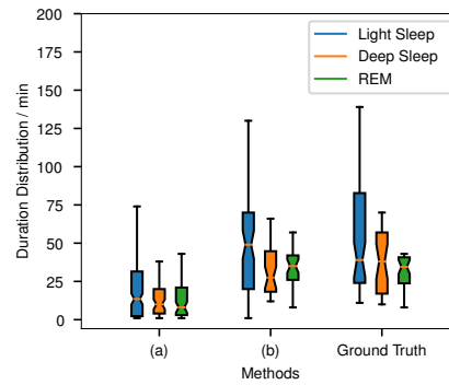
Fig. 16. Duration distribution of each stage, (a) CNN-BiLSTM method without duration constraint, (b) CNN-BiLSTM method with duration constraint.
