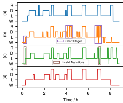
Fig. 15. Sleep stage classification results during the whole night, (a) Ground truth sleep stages, (b) CNN-BiLSTM method, (c) CNN-BiLSTM + duration constraint, (d) CNN-BiLSTM + duration constraint + transition constraint (full WiFi-Sleep).
