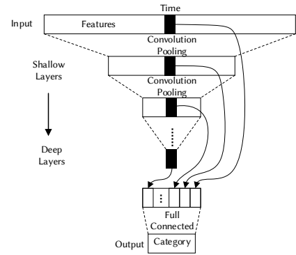
Fig. 12. Multi-scale CNN structure.
