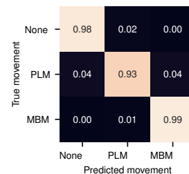
Fig. 20. Confusion matrix of body movement detection
