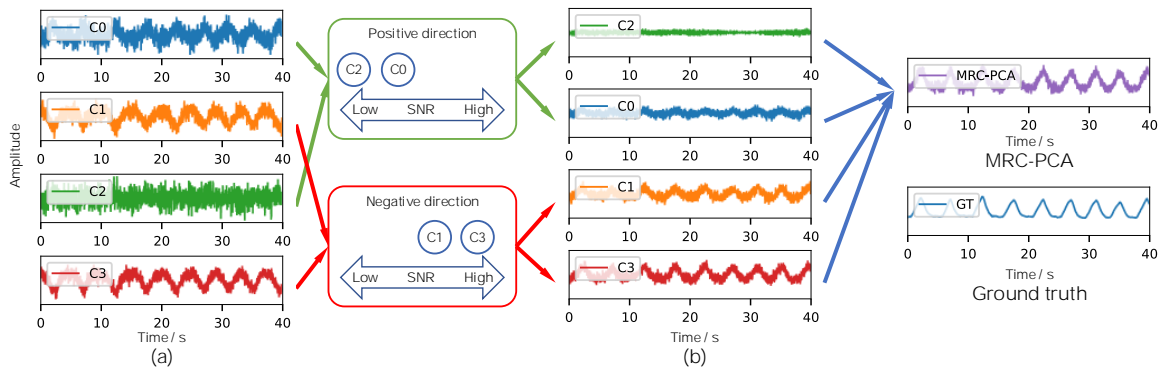
Fig. 3. a) Original signals with different SNRs and directions; b) Signals multiplied by gains from MRC-PCA.
