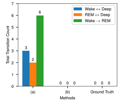
Fig. 17. Invalid sleep stage transition counts, (a) CNN-BiLSTM method without transition constraint, (b) CNN-BiLSTM method with transition constraint.
