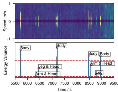
Fig. 5. Doppler-MUSIC speed spectrum and energy variance of speed spectrum and two thresholds.
