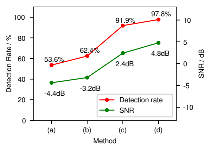
Fig. 18. Detection rate and SNR of different methods. (a) CSI, (b) MRC-PCA, (c) CSI ratio, (d) WiFi-Sleep (CSI ratio + MRC-PCA).
