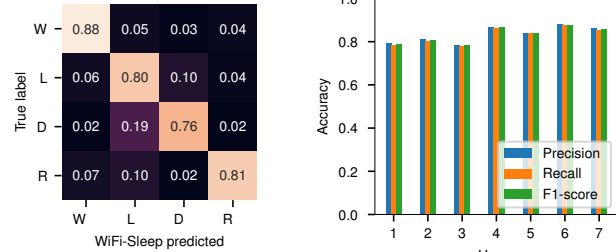
Fig. 14. a) Confusion matrix of WiFi-Sleep; b) Sleep stage classification performance of 7 users.
