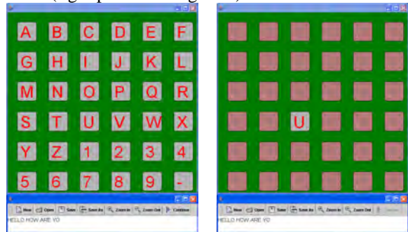
Figure 2. SD-Speller
