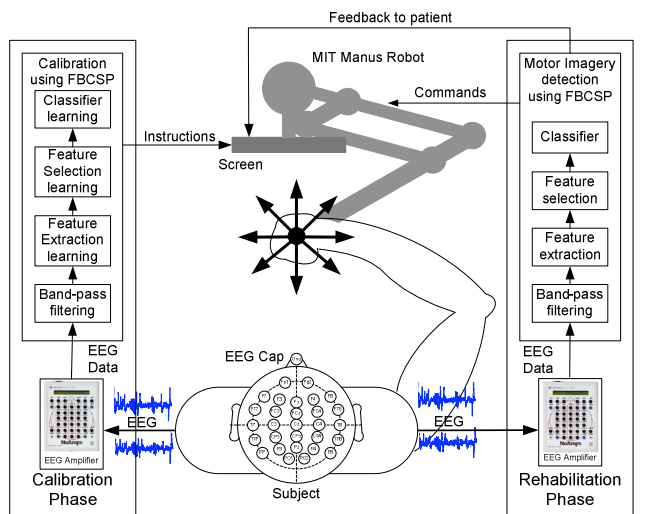
Fig. 1. Architecture of Motor Imagery-based Brain-Computer Interface (MI-BCI) for upper limb robotic rehabilitation
