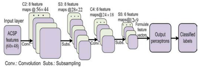
Fig. 2. Architecture of proposed CNNs-eeNet, each plane is a feature map, whose weights are to be identical.
