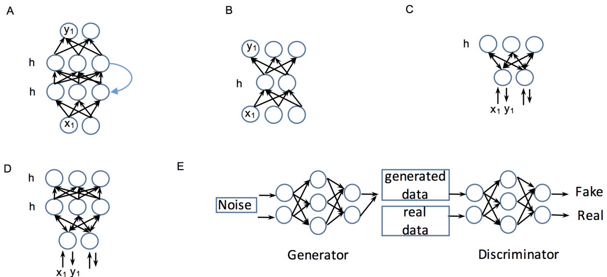
FIGURE 3. Various neural network architectures. A. Recurrent neural network, B. Autoencoder, C. Restricted Boltzmann Machine, D. Deep Belief Network, E. Generative Adversarial Network. x , y , h represent input, output and hidden layers respectively.
