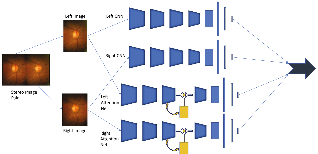
Fig. 1. An overview of our attention-guided stereo ensemble network (AGSE-Net). The elements in blue represents ResNet CNN backbone for feature extraction. The elements in grey represent the classifier modules in the CNNs. The elements in yellow represent visual attention localization modules. The large arrow at the right end of the figure decides the overall output of the ensemble based on the output of each of the four branch networks. In the present work, the output of each branch represents the likelihood for positive or negative in glaucoma screening and the highest value determines the screening outcome. The input stereo image pair is first split into left and right images, each of which is fed into the respective CNN and attention net, and the results are then combined as an ensemble at the end to calculate prediction scores. For both the CNN and the Attention Network, the Global Average Pooling layer after the convolution layers are maintained. ResNet-34 [48] is selected as the CNN in this paper, due to its effective error-propagation, excellent performance, and yet reasonable computational load. (For interpretation of the references to color in this figure legend, the reader is referred to the web version of this article.)
