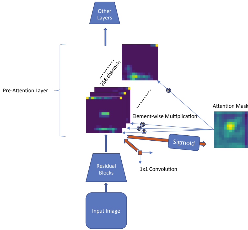
Fig. 2. The structure of the attention network.
