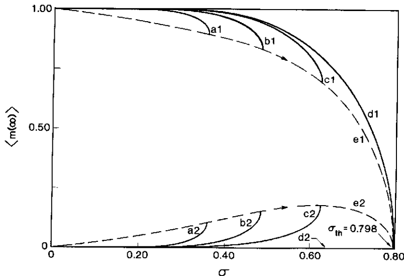
FIG. 1. Solid lines labeled a–d are the average overlaps between the final state of network A and the two patterns S^1 and S^2 , for projection strengths \lambda = 0.34, 0.20, 0.08 , and 0 , respectively, for case i and \lambda < \lambda_c as a function of \sigma , the noise level. Numerals 1 and 2 represent the corresponding overlaps with patterns S^1 and S^2 , respectively. Dashed lines labeled e are the envelopes of the overlap curves at noise thresholds for different projection strengths \lambda . Arrows on these dashed lines indicate the directions in which \lambda decreases ( 0 \leq \lambda \leq 1 ). The noise thresholds for curves a–d are \sigma_\lambda = 0.360, 0.483, 0.624 , and 0.798 , respectively.
