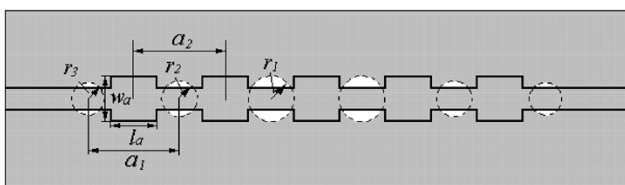
Fig. 7. Schematic of the ground-tapered C-EBG structure adopting the Chebyshev distribution.
