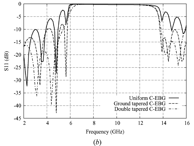
Fig. 9. Simulated S-parameters of the tapered and uniform dual-plane C-EBG microstrip structure. (a) S_{21} . (b) S_{11} .
