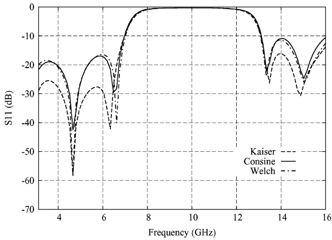
Fig. 5. Simulated S_{11} parameters of tapered 1-D EBG microstrip structures in Group Two.
