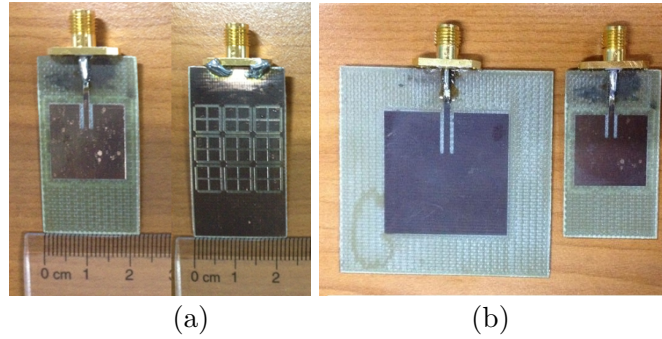
Figure 6. The photos of microstrip antenna. (a) The top view and back view of proposed antenna. (b) The proposed antenna vs. the conventional patch antenna.
