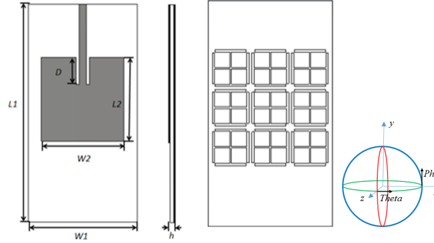
Figure 3. The illustration of microstrip antenna.
