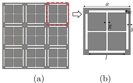
Figure 1. (a) Pattern ground plane of the metasubstrate. (b) Unit cell of the etched uni-planar compact structure. a = 7mm , l = 5.5mm , w = 0.4mm , and g = 0.25mm .
