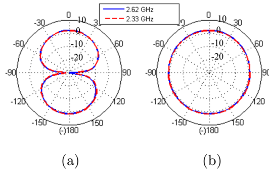
Figure 11. The radiation patterns with varied inductance. (a) E-plane. (b) H-plane.
