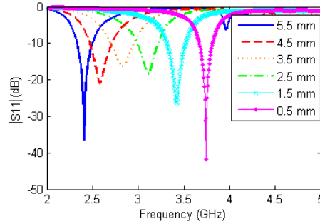
Figure 7. The dependence of reflection coefficients on parameter l .
