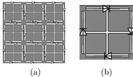
Figure 9. The equivalent circuit of the tunable antenna. (a) the pattern in the ground plane. (b) one unit cell with diodes.
