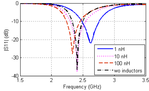
Figure 10. The simulated result of the tunable antenna.
