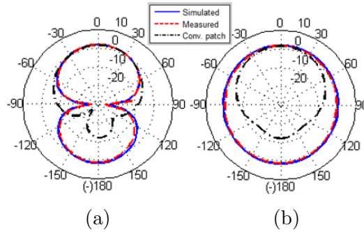
Figure 5. The simulated and measured radiation pattern. (a) E-plane. (b) H-plane.
