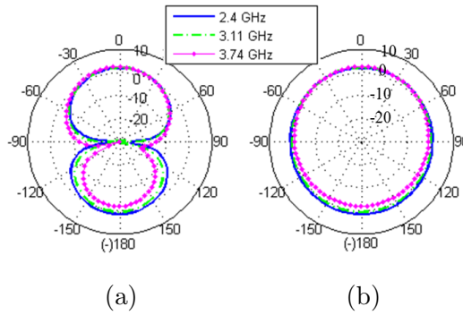
Figure 8. The radiation patterns with varied l . (a) E-plane. (b) H-plane.
