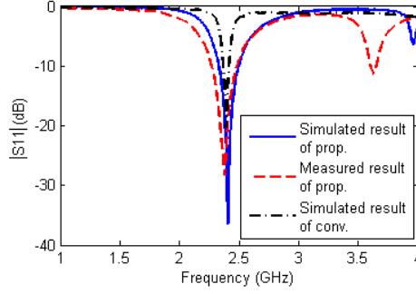
Figure 4. The simulated and measured return loss.
