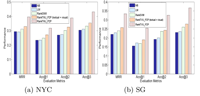
Figure 7: Performance comparisons.
