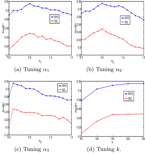
Figure 6: Parameter tuning.
