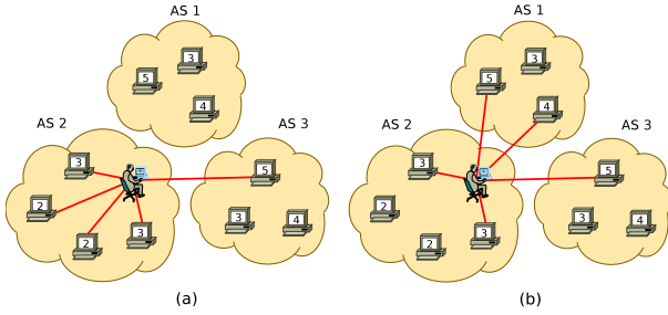
Fig. 2. Demonstration of the tradeoff between traffic locality and streaming quality guarantee. The number in each PC icon means the upload capacity. Assuming download rate 20 is required for an uninterrupted stream, the partnership in (a) cannot satisfy the rate requirement whereas the partnership in (b) can.
