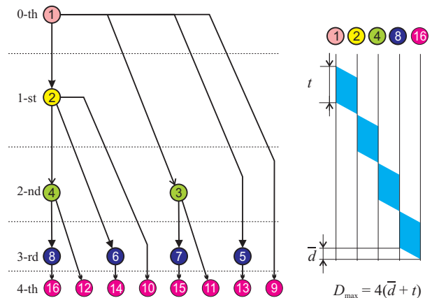
Fig. 3. The SBT of single chunk dissemination. We illustrate both maximum delay calculation and the geometric progression nature of R_k in the figure.
