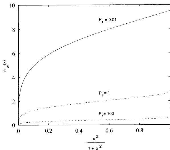
Fig. 5. Variation of \theta_w(x) , calculated from Eq. (46), with Prandtl number Pr for the case m = -1/4 (corresponding to a uniform wall temperature for large x ).
