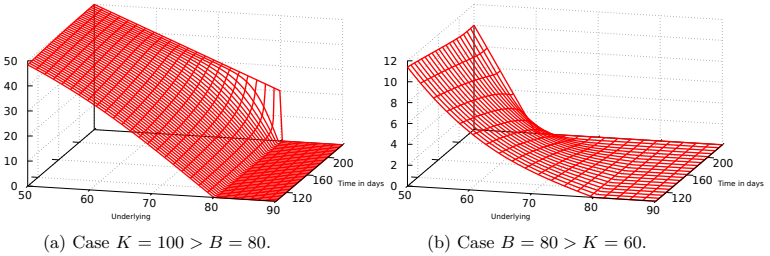
Fig. 11.2: Graphs of the up-and-out put option prices (11.8)-(11.9).
