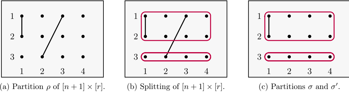
Figure 9: Splitting of a partition \rho into \sigma and \sigma' with n = 2 and r = 4 .
