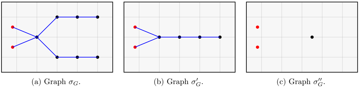
Figure 12: Splitting of \rho_G into \sigma_G and \sigma'_G with n = 2 , r = 4 and two endpoints m = 2 . Then, \sigma''_G contains m endpoints in addition to at least one non-endpoint vertex due to the connectedness of \rho , hence we have v(\sigma''_G) \geq m + 1 . Since \sigma''_G \subset \sigma'_G and v(\sigma''_G) \geq m + 1 , by the balance condition (2.6) we have
