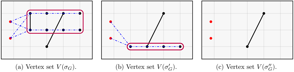
Figure 11: Splitting of V(\rho_G) into V(\sigma_G), V(\sigma'_G) with n = 2 , r = 4 and two endpoints m = 2 .
