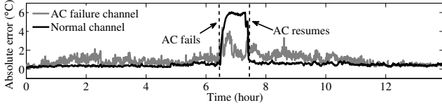
Figure 10. Average absolute temperature prediction error (prediction horizon = 5 minutes)
