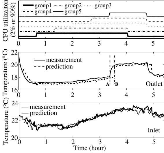
Figure 7. Top: CPU utilization of testing data. Middle: temperature measurements and predictions at an outlet of Group 5 with 10 minutes prediction horizon. Bottom: temperature measurements and predictions at an inlet of Group 3 with 10 minutes prediction horizon.
