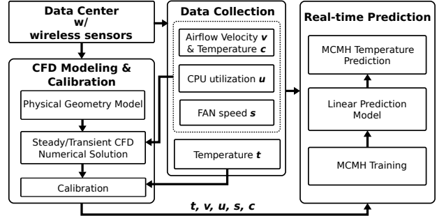
Figure 1. Prediction system architecture.
