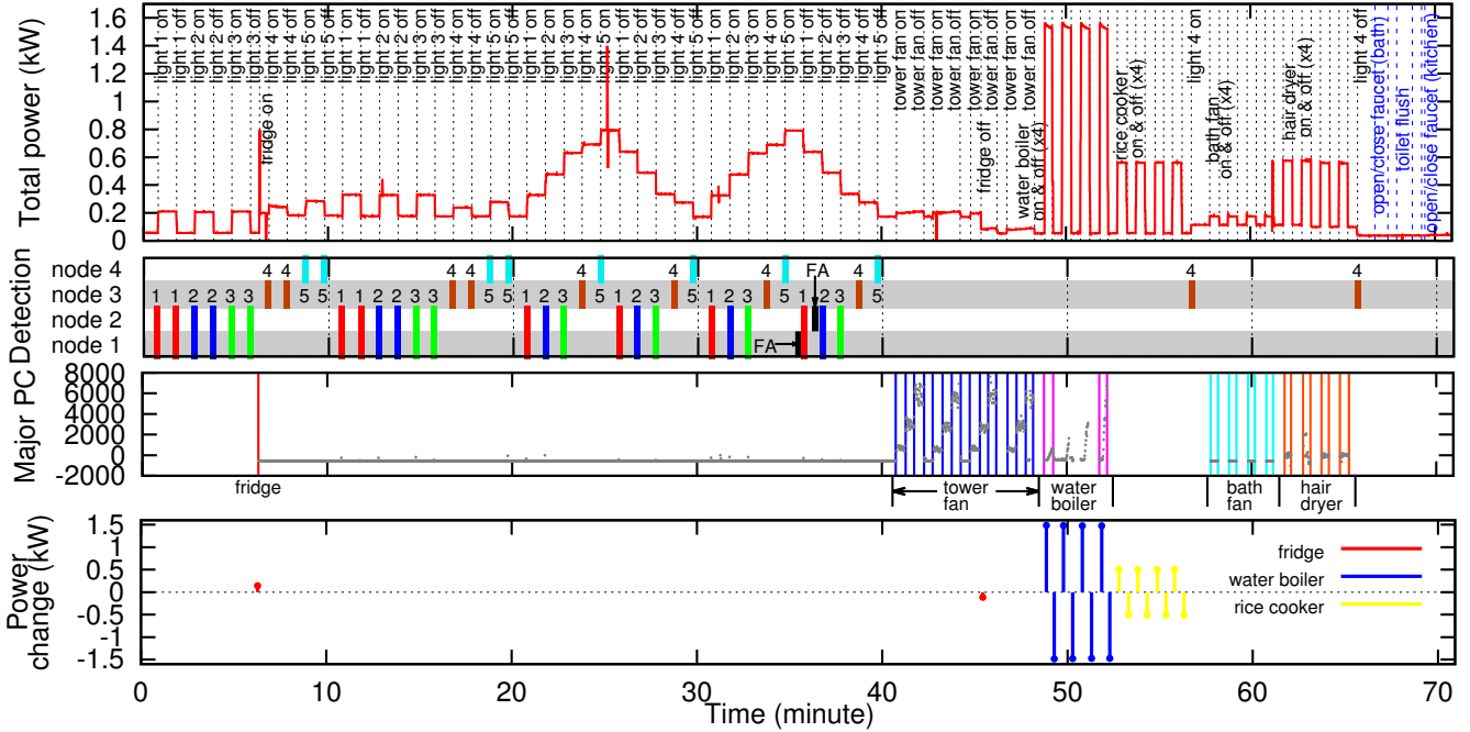
Fig. 6. Results of the controlled experiment in Apartment-1. (1) The top chart shows the power readings labeled with ground truths of the events. (2) The bars in the second chart show the detections of the light sensors. Two black bars at around the 35 th minute are false alarms (labeled “FA” in the chart) identified by the multi-modal data correlation. Clusters are differentiated by colors and the overhead numbers are the IDs of the associated light. (3) The third chart shows the major principle component given by PCA and the detected acoustic transitions. The acoustic transitions of the same color are associated with the same appliance. (4) The bottom chart shows the clustered and associated power events of the unattended appliances.
