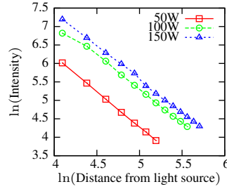
Fig. 4. Light intensity vs. distance (centimeters) in log-scale.
