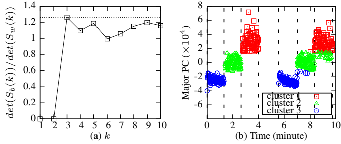
Fig. 5. Acoustic event clustering and transition detection for a 3-speed fan. (a) The number of phases is identified as three; (b) Clustering and transition detection results, where Y-axis is the major principle component (PC) and vertical lines represent the detected acoustic transitions.
