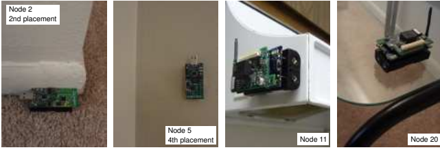
Fig. 9. Sensor installation examples. Sensors were placed on the ground, in the corner of walls, on the fan of a range, and on a table.
