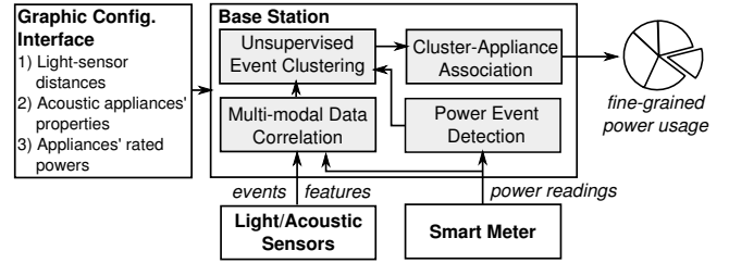
Fig. 1. The Supero architecture.
