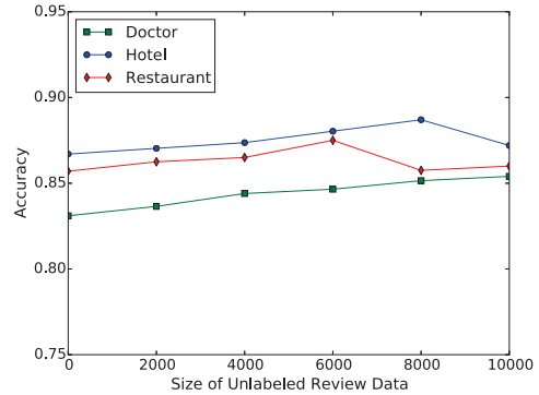
Figure 1: Accuracy versus Unlabeled Data Size.
