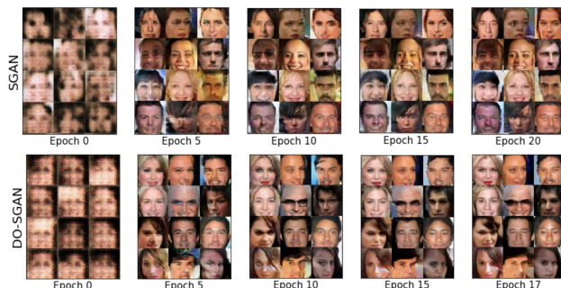
Figure 1. Training images with fixed noise for SGAN and DO-SGAN/P (pruning) until termination. Both during training and after convergence, DO-SGAN/P can generate better quality images with FID score of 6.32 against SGAN's FID score of 6.98.
