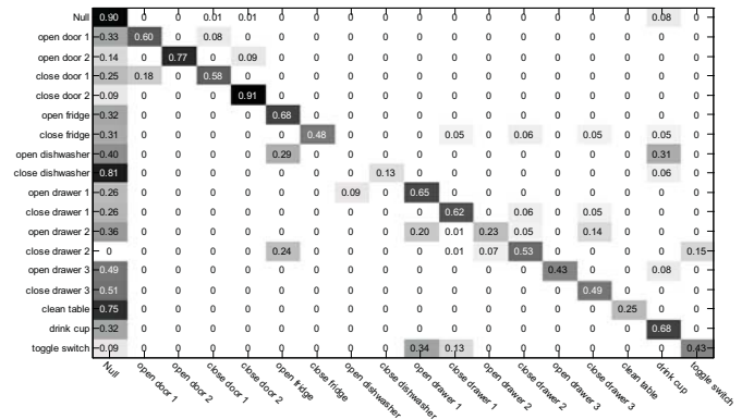
Figure 3: Confusion matrix yielded by the proposed CNN method (without temporal smoothing) on the Opportunity Activity Recognition dataset for Subject 1 (the larger the value the darker the background).
