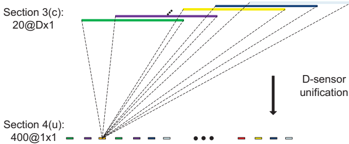
Figure 2: Illustration of unification layer ( i.e. the fourth section in Figure 1).
