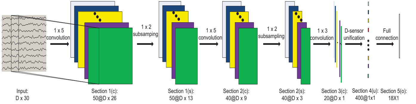
Figure 1: Illustration of the CNN architecture used for a multi-sensor based human activity recognition problems. We use the Opportunity Activity Recognition dataset presented in Section 4 as an illustrative example. The symbols “c”, “s”, “u”, “o” in the parentheses of the layer tags refer to convolution, subsampling, unification and output operations respectively. The numbers before and after “@” refer to the number of feature maps and the dimension of a feature map in this layer. Note that pooling, ReLU and normalization layers are not showed due to the limitation of space.
