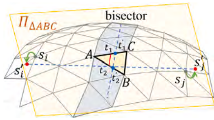
Fig. 6. Refine ordinary GVD segments. Let \Pi_{\Delta ABC} be the plane of \Delta ABC . s_i (resp. s_j ) is unfolded onto \Pi_{\Delta ABC} according to d(t_1; s_i) and d(t_2; s_i) (resp. d(t_1; s_j) and d(t_2; s_j) ), yielding an image point s'_i (resp. s'_j ). The two images s'_i and s'_j can fine-tune the GVD segment to a better configuration.
