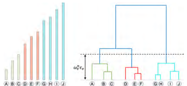
Fig. 6. Hierarchical clustering of (left) 10 edges and (right) the resulting dendrogram. The horizontal dashed line shows the prescribed tolerance \omega_e^n \epsilon_e , resulting in three clusters of edges.
