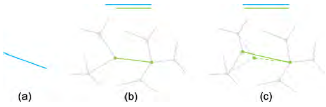
Fig. 10. Vertex perturbation to reassign (b) an edge (in green) to a cluster whose (a) centroid (in blue) has a similar length to the edge. (c) Perturbing one end (i.e., the left end) of the edge makes the edge’s length closer to that of the centroid.
