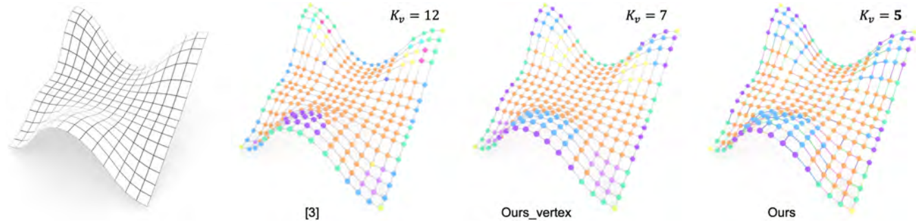
Fig. 16. Comparing [3] with our approach (Ours) as well as a variation of our approach (Ours_vertex) to model a quad mesh with discrete equivalence classes of vertices. The input surface is shown on the left and statistics of the three results are provided in Table III.
