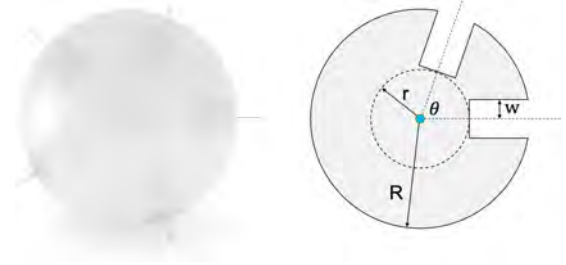
Fig. 3. Modeling the geometry of a node corresponding to a mesh vertex with valence 5, where the vertex is at the center of the node and each incident edge defines a cylindrical hole on the node. A cross-section of the node is shown on the right, where the cross-section plane passes through two cylindrical holes on the node.
