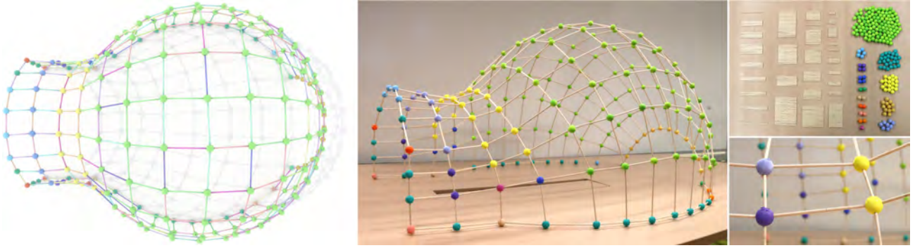
Fig. 1. An IGLOO surface with an original mesh containing 196 vertices and 364 edges optimized to 14 classes of vertices and 30 classes of edges using our approach. Left: a rendering of our optimized wireframe mesh, where vertices and edges in the same class are rendered with the same color, respectively. Middle: fabricating the wireframe mesh with 3D printed nodes and precision-cut wooden rods. Right: (top) nodes and rods of the same class are clustered together, and (bottom) a close-up view of the assembled nodes and rods.
