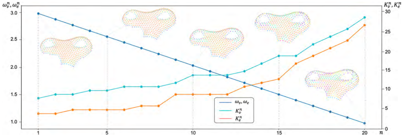
Fig. 14. Our computational framework iteratively clusters and optimizes the mesh to discover new clusters of vertices and edges ( K_v^n, K_e^n ) guided by the two prescribed tolerances ( \omega_v^n, \omega_e^n ) that are gradually decreased in each iteration.
