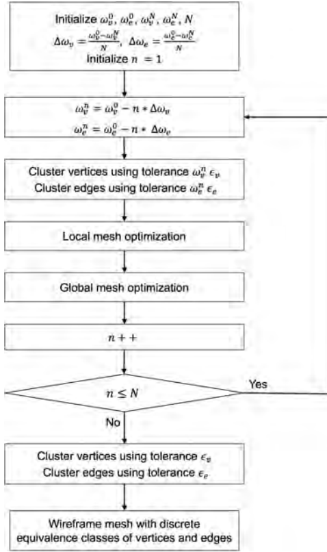
Fig. 5. A diagram of our computational framework to model wireframe meshes with discrete equivalence classes.
