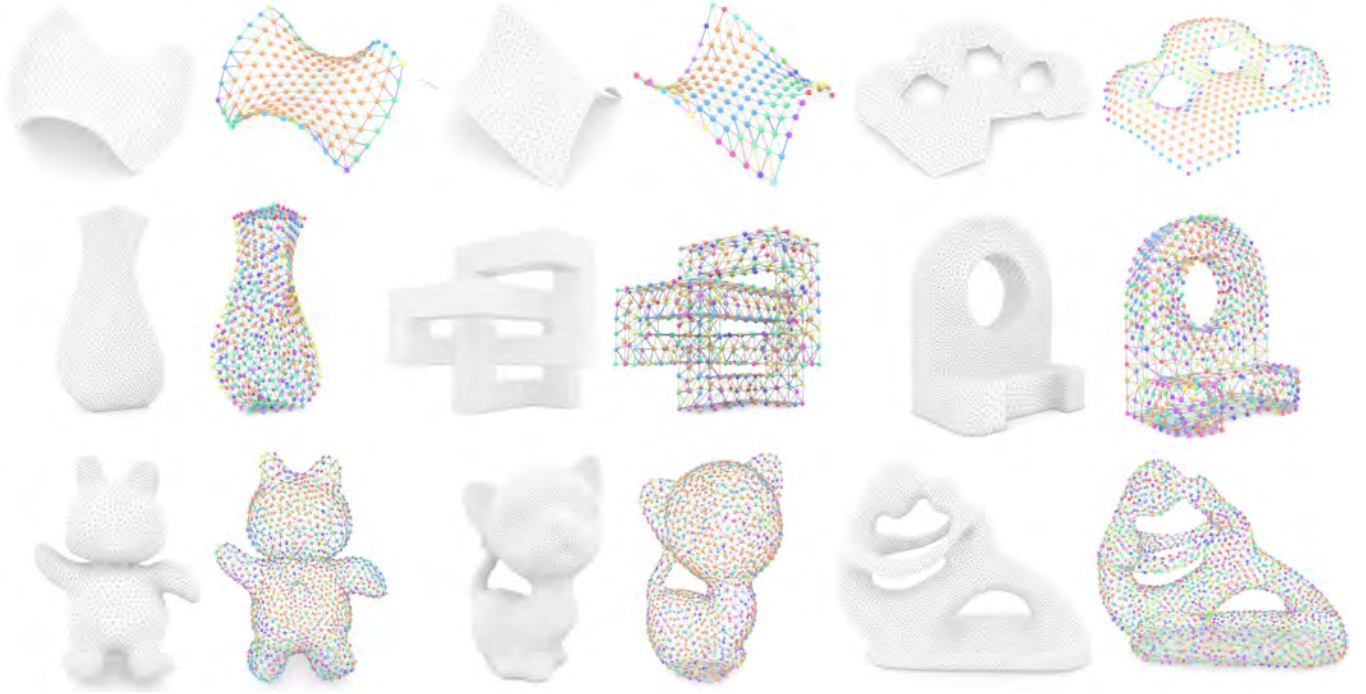
Fig. 12. Our approach allows modeling wireframe meshes with discrete equivalence classes for surfaces with various shapes and topologies. From left to right and then top to bottom: FLOWER, MONKEY SADDLE, FREE HOLES, VASE, KNOT, CAD PART, TEDDY, KITTEN, and FERTILITY. The input surface \mathbf{P} is also shown beside each result.
