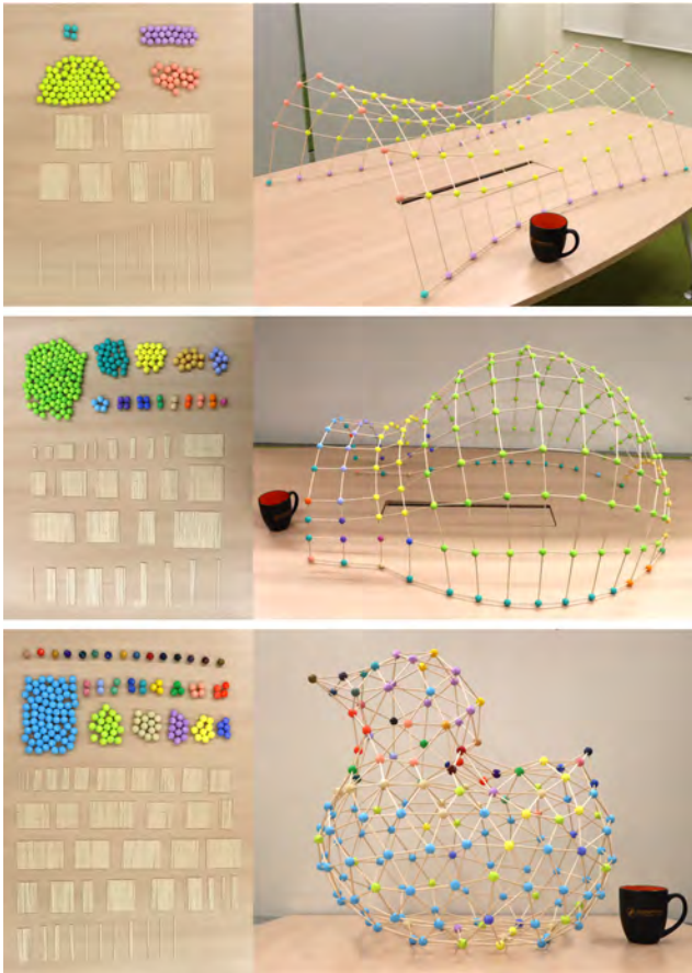
Fig. 19. We fabricate three of our modeled wireframe meshes with 3D printed nodes and precision-cut rods, from top to bottom, HYPERBOLIC, IGLOO, and DUCK. Fabricated nodes and rods of the same class are clustered together on the left. A mug is put beside each structure to show its real scale.
