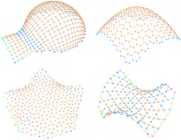
Fig. 13. Our approach allows modeling wireframe polygonal meshes with different patterns, including quad, hexagon, triangle-quad, and triangle-hexagon patterns.
