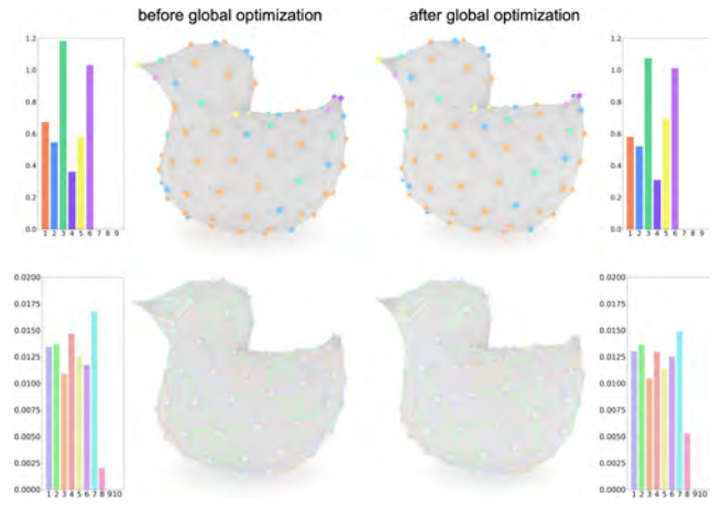
Fig. 11. (Top) 9 vertex clusters and (bottom) 10 edge clusters in a DUCK model (left) before and (right) after our global mesh optimization to reduce intra-cluster variance. The intra-cluster variance of each vertex/edge cluster is shown as a histogram beside the corresponding model. Note that vertex clusters and edge clusters are sorted according to the cluster size in descending order, respectively. The 7th, 8th, and 9th vertex clusters only have a single vertex and thus they do not have intra-cluster variance (i.e., no bar in the top histograms). The same applies to the 9th and 10th edge clusters.
