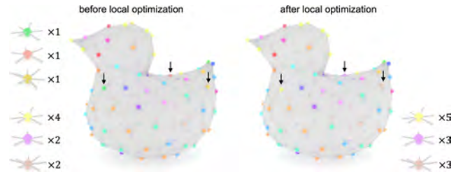
Fig. 9. Clustering of vertices (left) before and (right) after running our local mesh optimization to eliminate clusters with few vertices. Three clusters, each of which has a single vertex, eliminated by our vertex perturbation are shown on the top left corner, and also highlighted with black arrows in the mesh on the left. The centroids of three clusters to assign the three vertices, respectively, are shown at the bottom.
