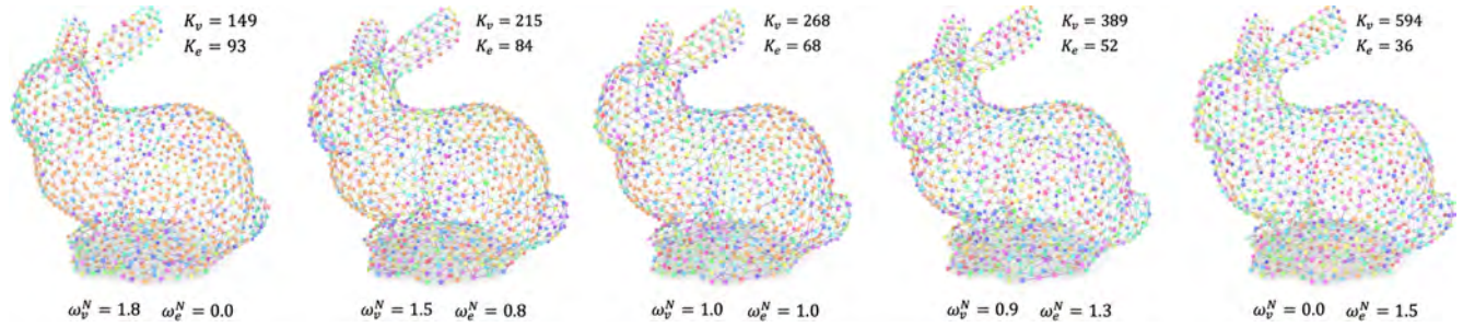
Fig. 15. Our approach allows users to specify their preference on reducing the number of distinct vertices or edges, by setting the values of \omega_v^N and \omega_e^N . We show the number ( K_v ) of vertex classes and the number ( K_e ) of edge classes beside each resulting mesh.
