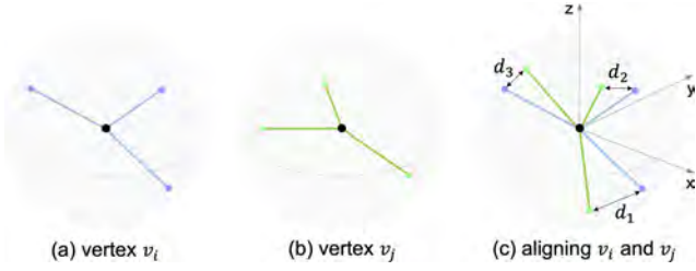
Fig. 7. We measure the shape dissimilarity of two vertices (a) v_i and (b) v_j with valence 3 by (c) finding the best alignment transformation that minimizes the sum of squared distances (i.e., d_1 , d_2 and d_3 in this example) between corresponding neighboring vertices projected onto a unit sphere.
