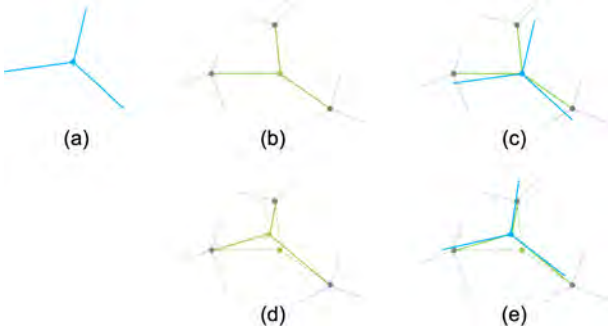
Fig. 8. Vertex perturbation to reassign (b) a vertex (in green) to a cluster whose (a) centroid (in blue) has (c) a similar shape. (d&e) Vertex perturbation makes the vertex’s shape closer to that of the centroid, yet it may also modify the shapes of neighboring vertices (in black) and the lengths of incident edges (in green).
