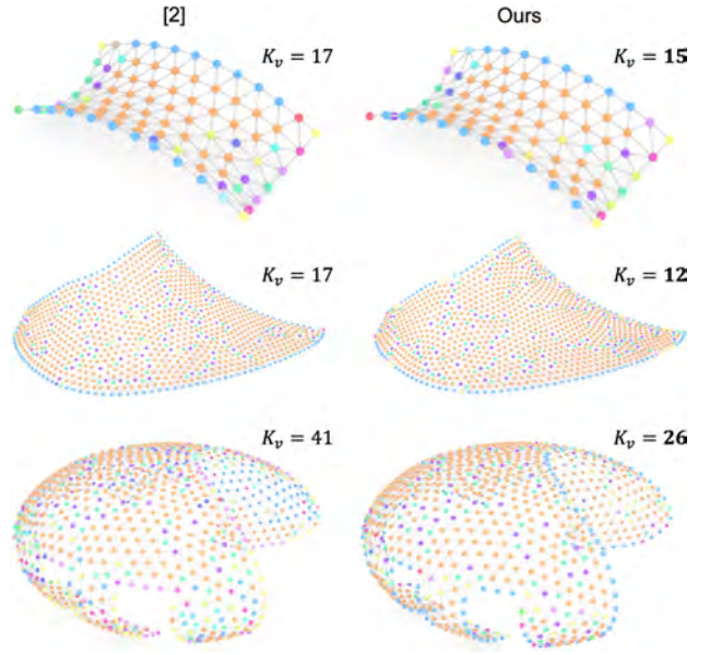
Fig. 17. Comparing [2] with our approach to model three architectural surfaces with discrete equivalence classes of vertices, where our approach generates a smaller number ( K_v ) of vertex classes for each surface. Statistics of the results are provided in Table III.
