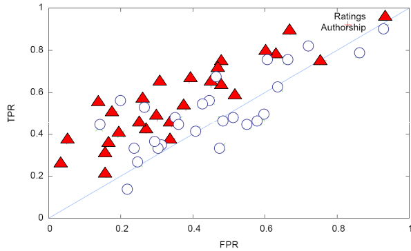
Figure 2: Performance of Bayesian credibility model
