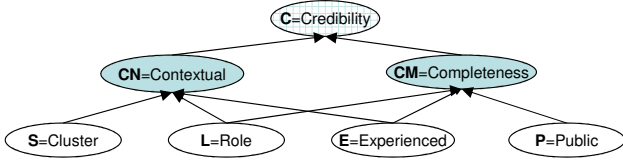
Figure 1: Credibility model
